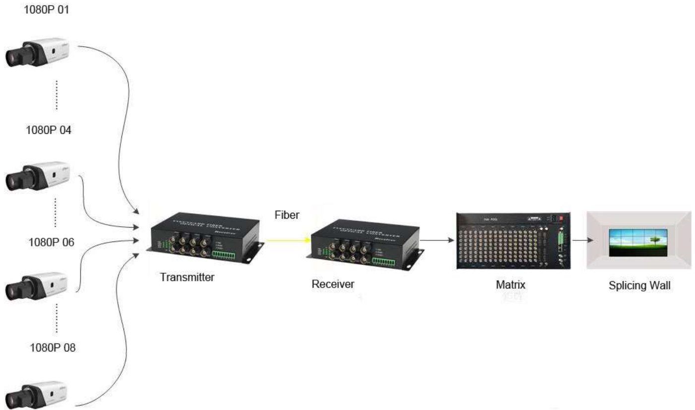
HD TVI/CVI/AHD/CVBS 720P/960P/1080P Series Connection Diagram
