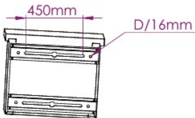
Figure 2 dimension support poteau-mural
