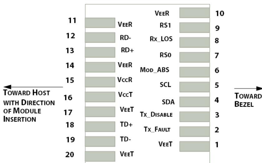
Figure1.Electrical Pin-out Details
